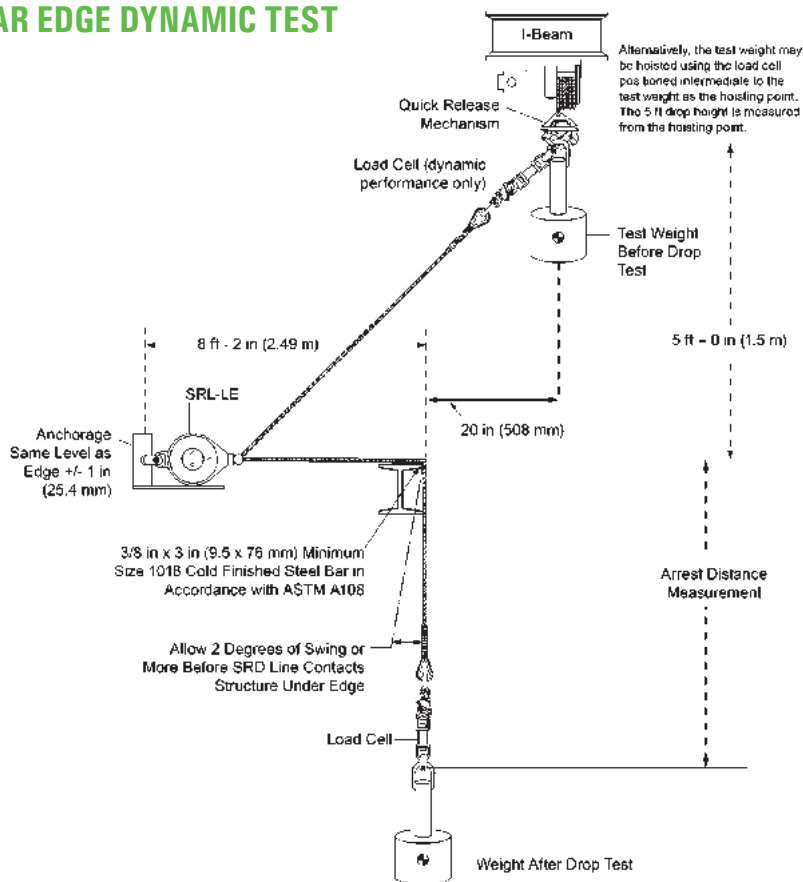
Figure 5b: Dynamic Performance Testing: SRL-Leading Edge
